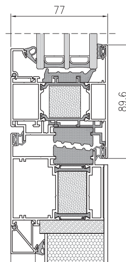
CROSS SECTION THROUGH TM 77HI PRESTIGE DOOR
