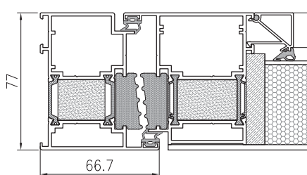
CROSS SECTION THROUGH TM 77HI PRESTIGE DOOR
